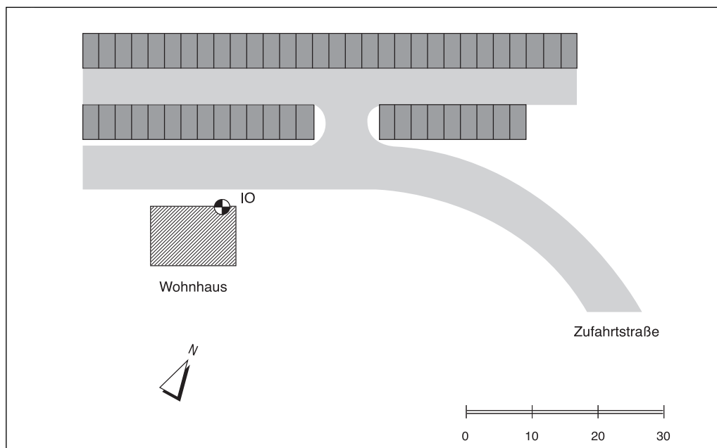
Fig. 38: Site plan for the calculation example of a company parking area containing 53 carports
