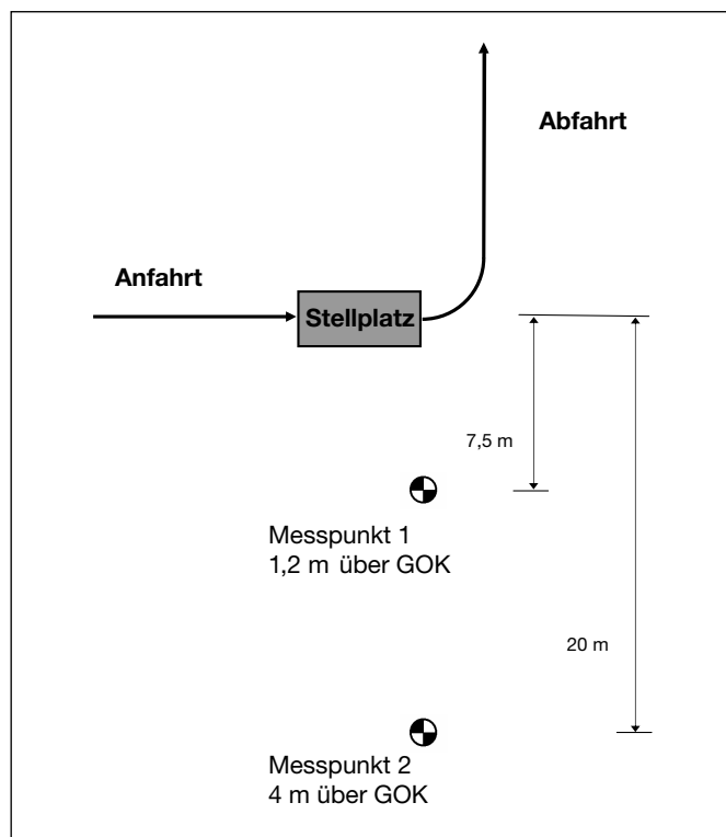
Fig. 19: Location outline of the sound level measurements of simulated parking processes of lorries
