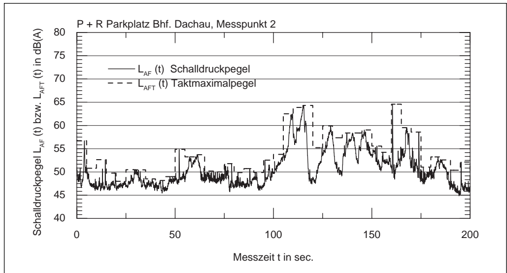
Fig. 35: Exemplary level-to-time diagram, controlling measurements
