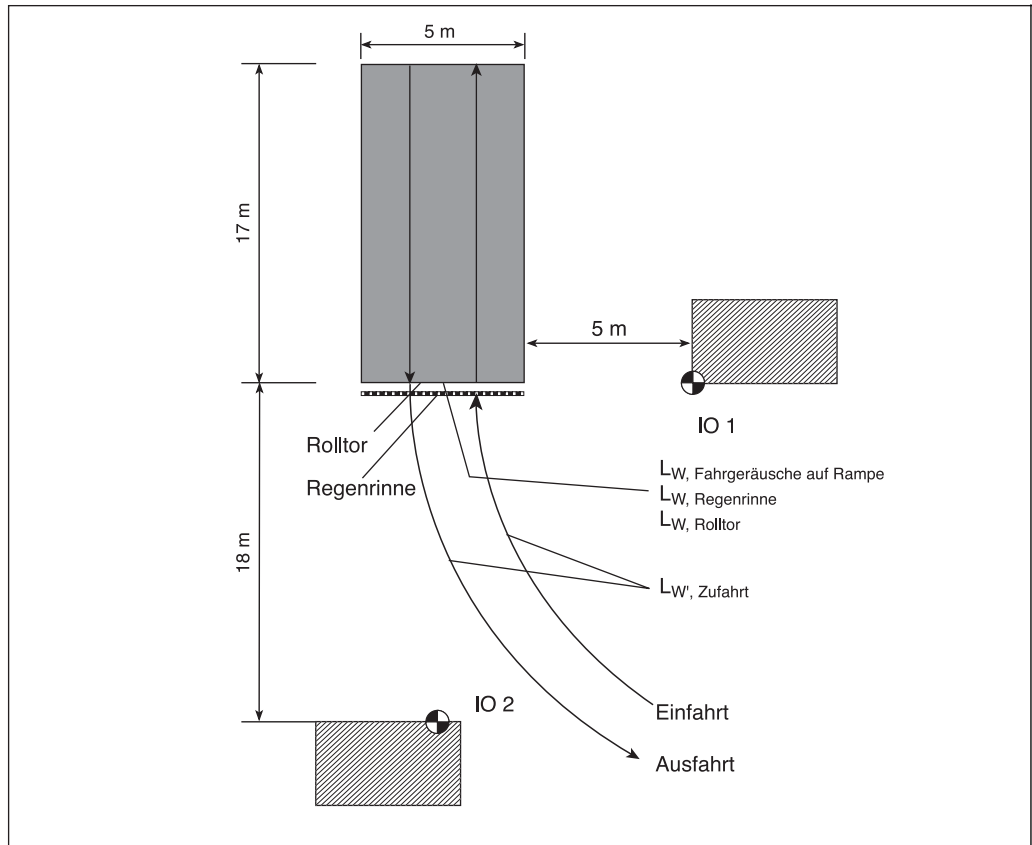
Fig. 40: Site plan for the calculation example of an enclosed underground car park ramp
