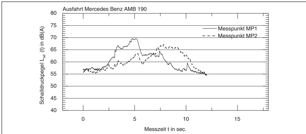
Fig. 24.2: Exemplary level-to-time diagram of a not enclosed underground car park ramp
