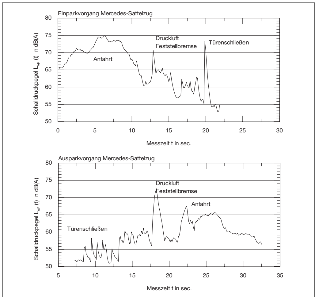
Fig. 20: Exemplary level-to-time diagrams of articulated lorries when leaving the carport (measuring point 20 m)
