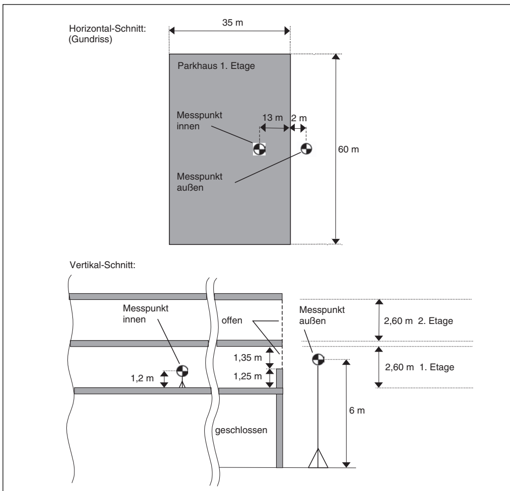
Fig 28: Location outline of the sound level measurements near an open multi-storey car park
