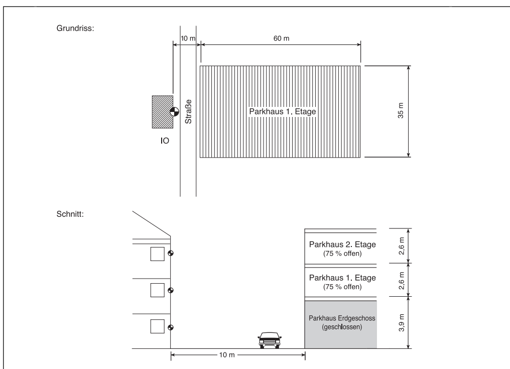
Fig. 41: Site plan and sectional view for the calculation example of an open multi-storey car park
