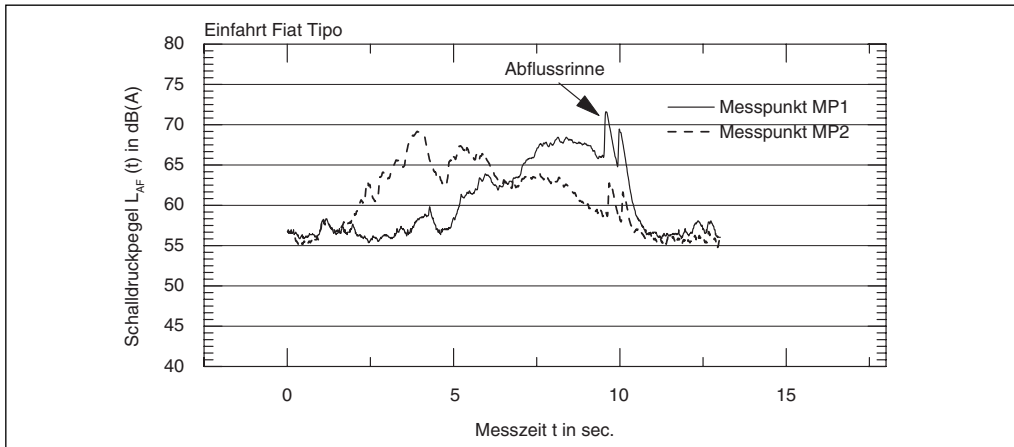
Fig. 24.1: Exemplary level-to-time diagram of a not enclosed underground car park ramp
