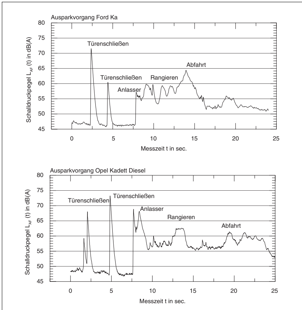
Fig. 17: Exemplary level-to-time diagrams of motorcars with Otto (petrol) and diesel engine when leav- ing the carport (measur- ing point 7.5 m)
