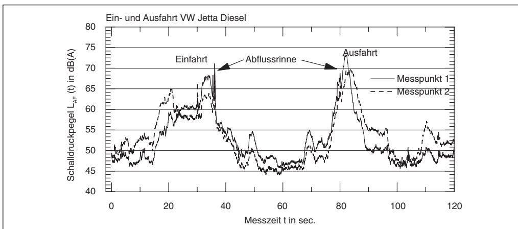
Abb. 24.3: Exemplary level-to-time diagram of a not enclosed underground car park ramp
