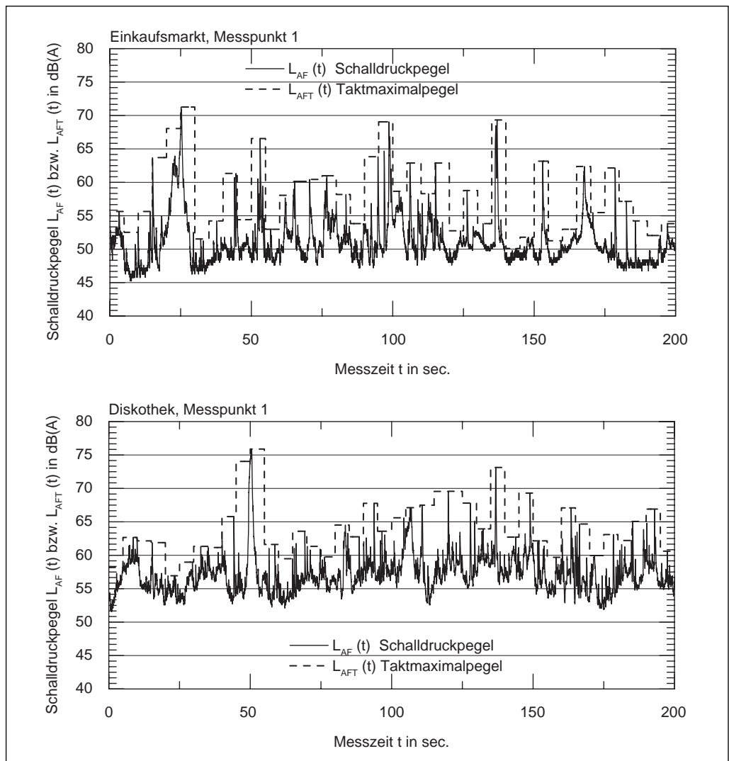
Fig. 36: Exemplary level-to-time diagrams, controlling measurements
