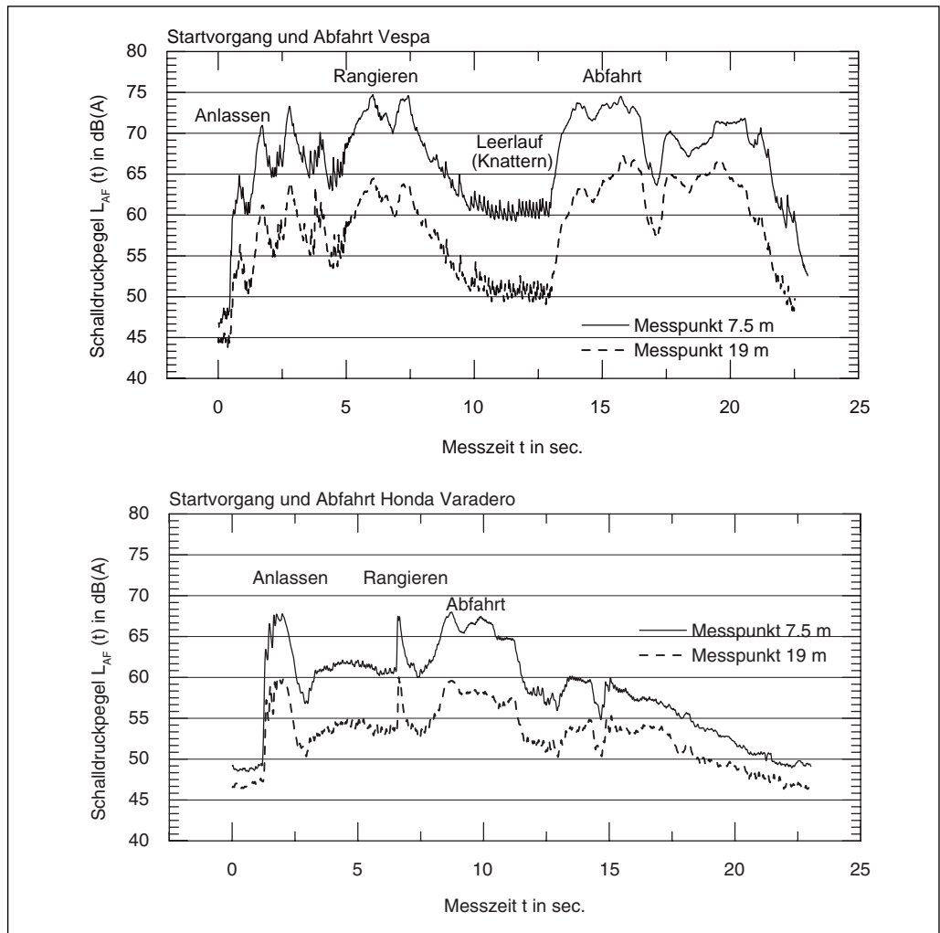
Fig. 18: Exemplary level-to-time diagrams of a scooter and of a motorcycle when leaving the carport (measuring points 7.5 m and 19 m)
