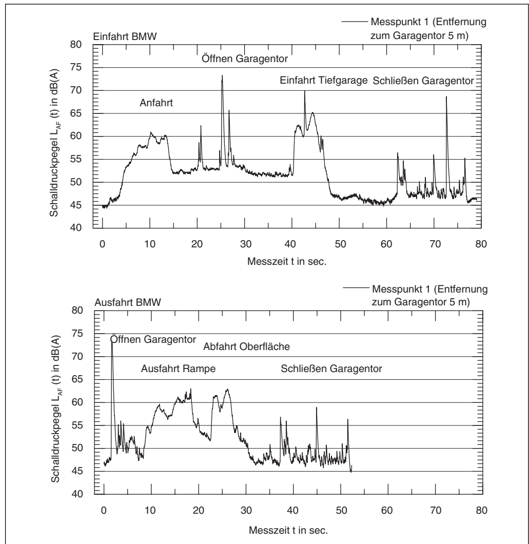
Fig. 25: Exemplary level-to-time diagrams near an enclosed underground car park ramp
