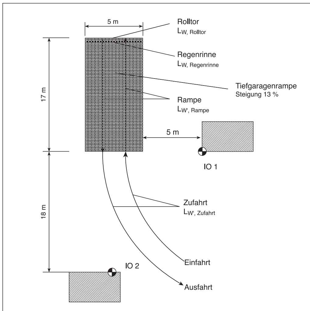
Fig. 39: Site plan for the calculation example of an open underground car park ramp
