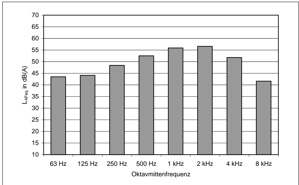
Fig. 29: Measurement in an open multi-storey car park – typical octave spectrum measuring point inside
