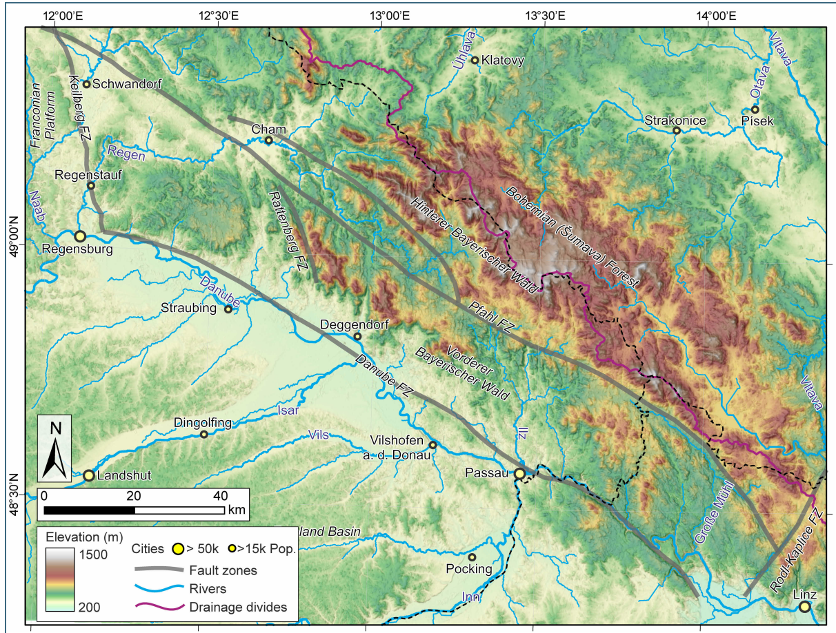
Fig. 2: Topographic map of the Bavarian Forest (from Copernicus GLO-30 DEM) along with main fault zones, main rivers, their tributaries, watershed divides, and cities. FZ; fault zone. The drainage divide is the continental drainage divide between the Danube River that drains into the Black Sea and Vltava, a tributary of Elbe River, that drains to the North Sea.
